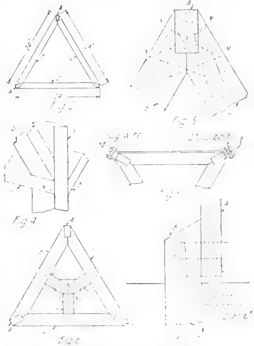
Diagram showing the construction of the built-up wireless mast
